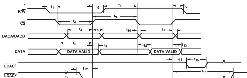
Figure 2. Timing Diagram
