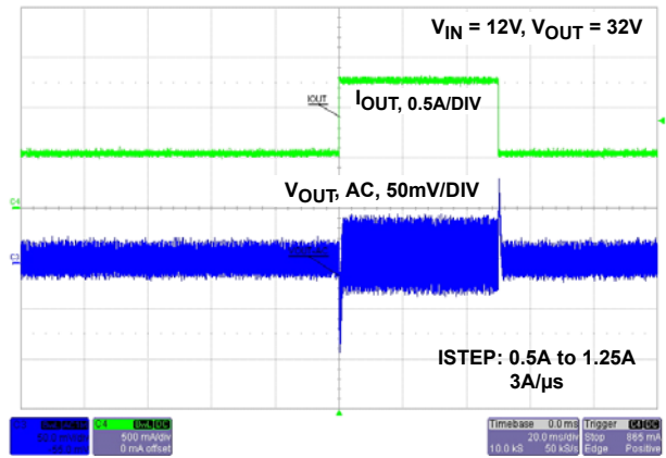
FIGURE 28. LOAD TRANSIENT, BOOST CONVERTER, INDUCTOR: WE 74477110; C_{OUT} : 2*220 \mu F 50V, 42m \Omega ESR
