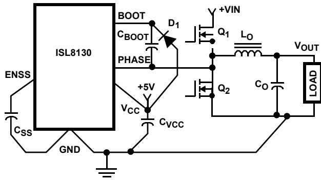
FIGURE 30. PRINTED CIRCUIT BOARD SMALL SIGNAL LAYOUT GUIDELINES
