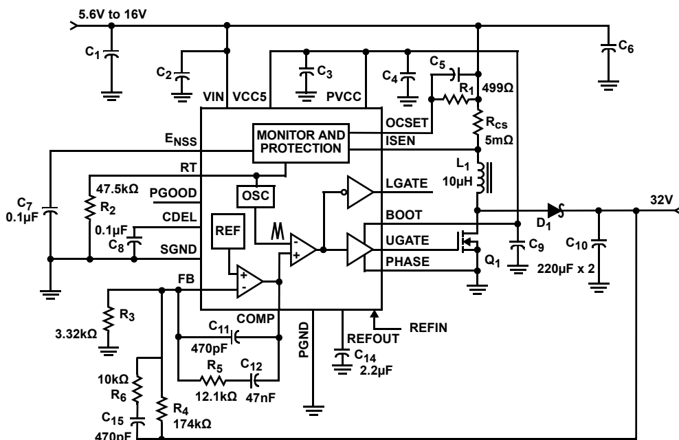
FIGURE 1. BOOST CONVERTER
