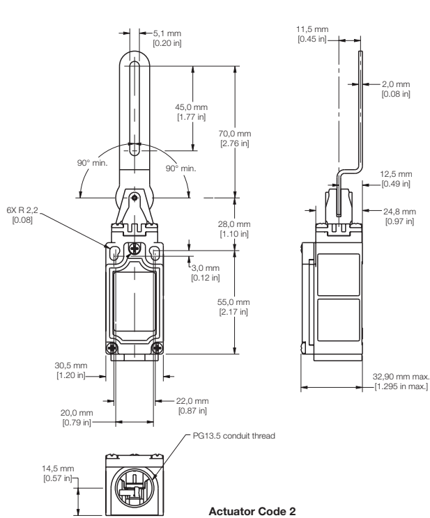
Figure 10. GSC/GSD Series with Hinge Overall Dimensions mm [in] Figure 11. GSE Series with Hinge Overall Dimensions mm [in]
