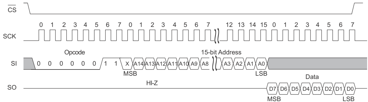
Figure 11. Memory Read
