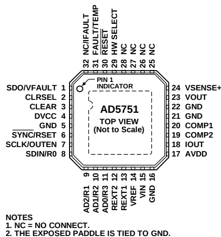
Figure 4. Pin Configuration
