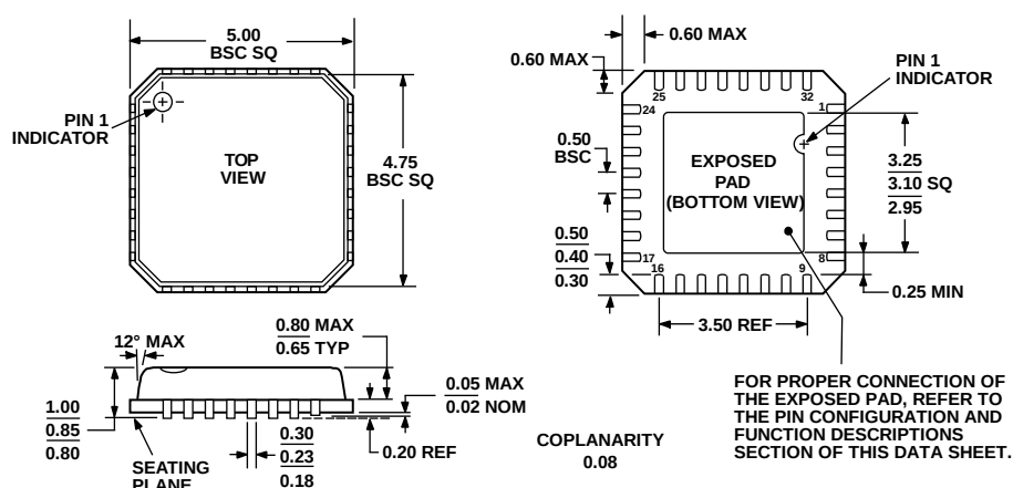
Figure 58. 32-Lead Lead Frame Chip Scale Package [LFCSP_VQ] 5 mm x 5 mm Body, Very Thin Quad (CP-32-2) Dimensions shown in millimeters
