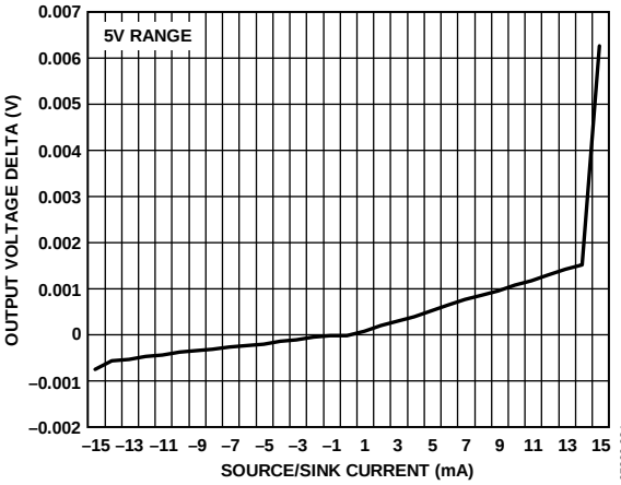
Figure 15. Source and Sink Capability of Output Amplifier
