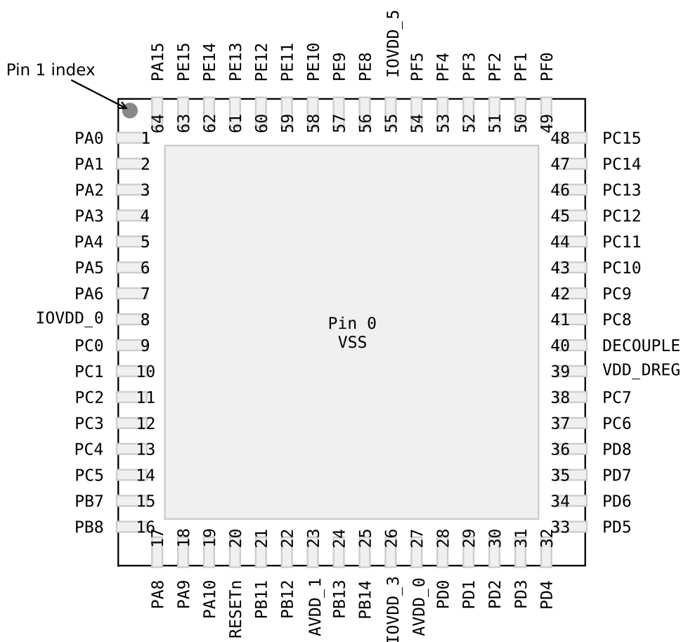
Figure 4.1. EFM32G230 Pinout (top view, not to scale)
