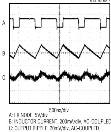
LIGHT-LOAD SWITCHING WAVEFORMS ( V_{IN} = +2.4\text{V} , V_{OUT} = +3.3\text{V} , I_{OUT} = 10\text{mA} )
