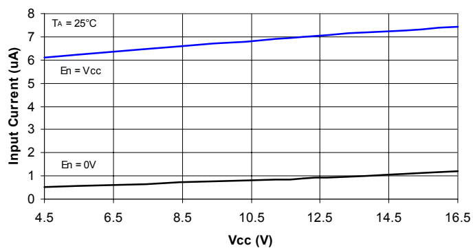
Input Current vs Vcc
