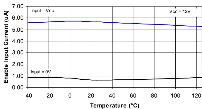
Enable Input Current vs Temperature
