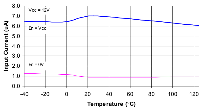
Input Current vs Temperature
