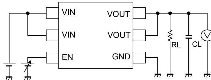
Fig.1 Measurement circuit
