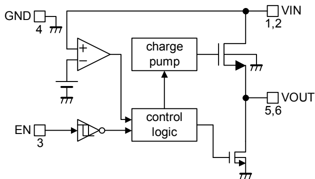
Fig.29 Block diagram
