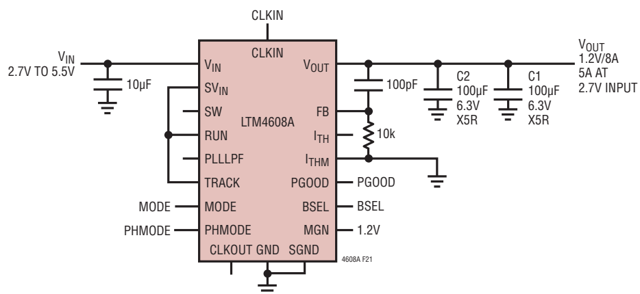
Figure 21. 2.7V to 5.5VIN, 1.2VOUT Design
