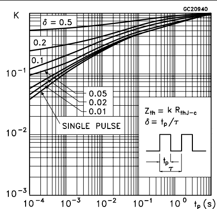
Figure 6. Safe operating area for DPAK, IPAK Figure 7. Thermal impedance for DPAK, IPAK
