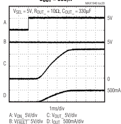
STARTUP TIME C_{OUT} = 330\mu F
