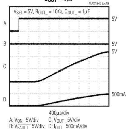
STARTUP TIME C_{OUT} = 1\mu F
