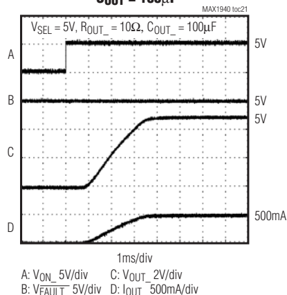
STARTUP TIME C_{OUT} = 100\mu F
