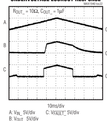
UNDERVOLTAGE LOCKOUT RESPONSE
