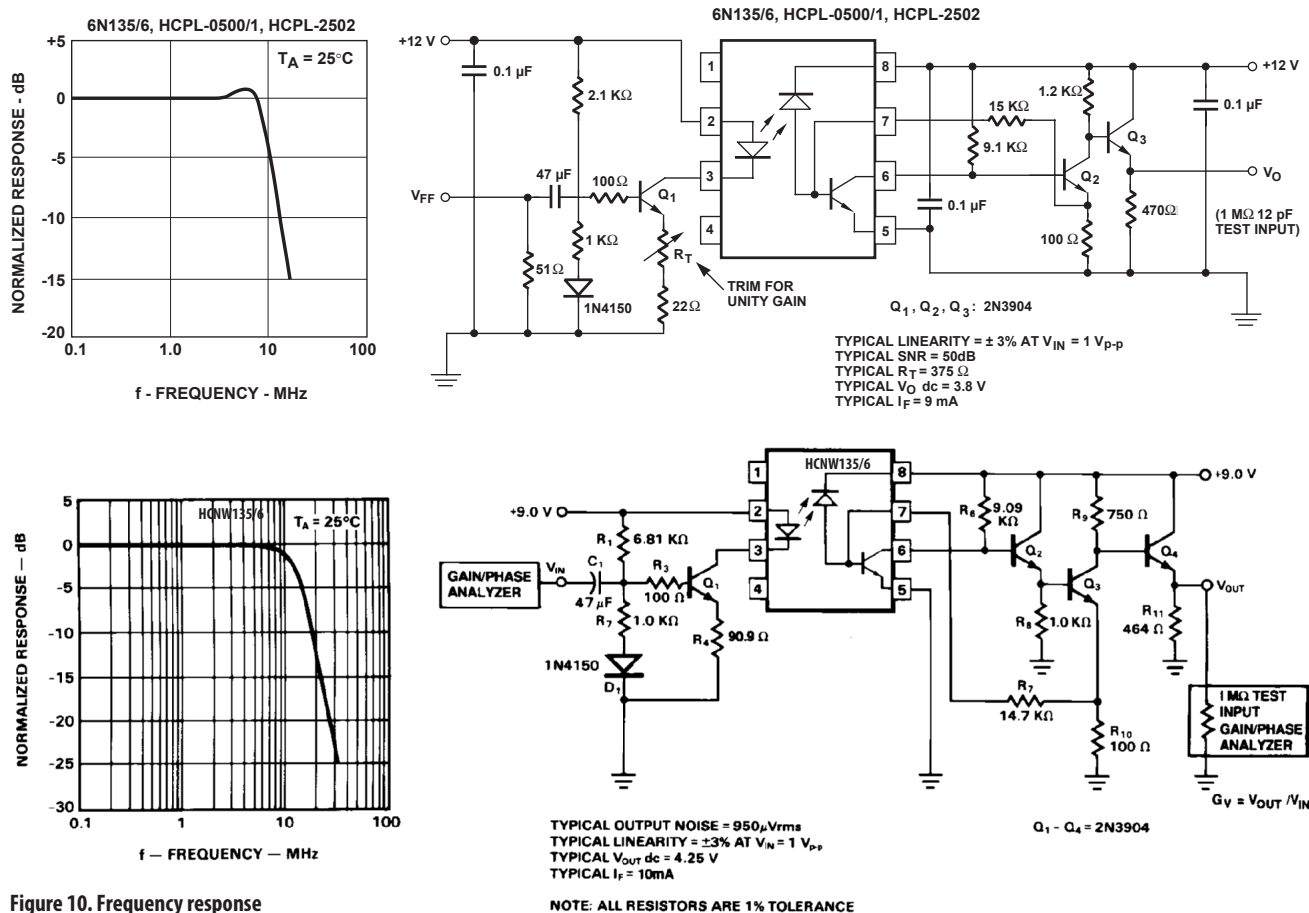
Figure 10. Frequency response
