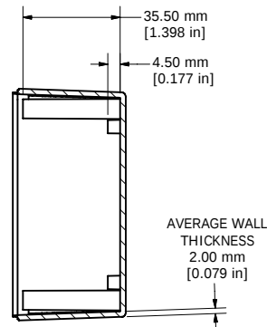
SECTION N-N
