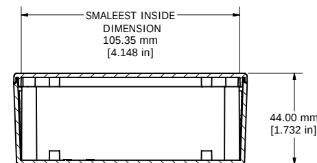
SECTION R-R
