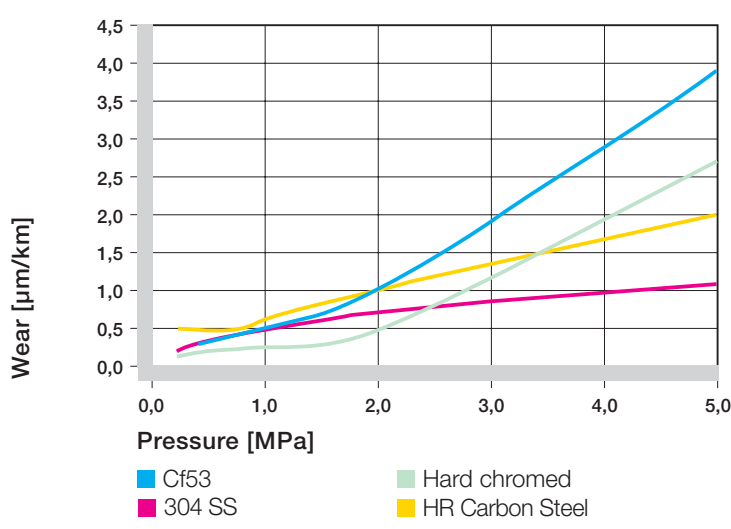
Graph 3.8: Wear of iglidur® J, rotating application with different shaft materials versus pressure
