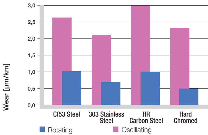
Graph 3.9: Wear for oscillating and rotating applications with different shaft materials under constant pressure, p = 2 MPa
