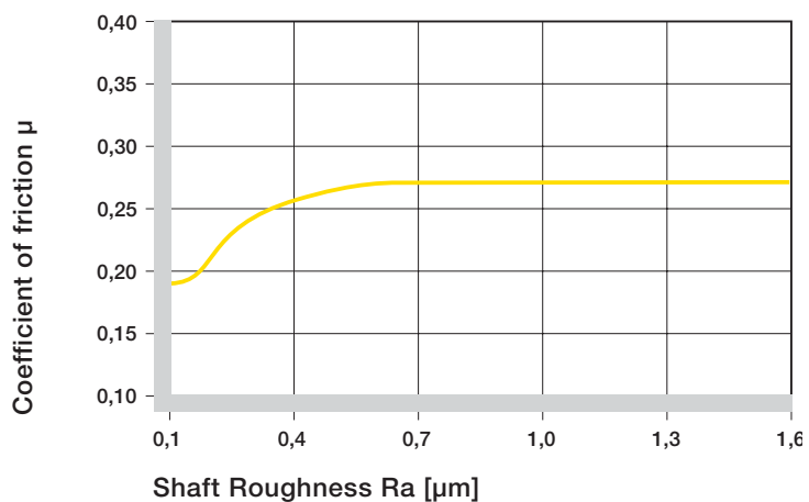
Graph 3.6: Coefficient of friction of iglidur® J as function of the shaft surface (Cf53 hardened and ground steel)
