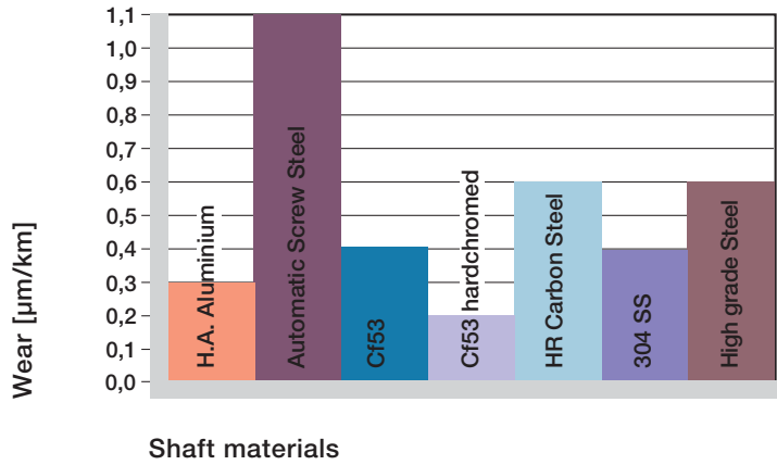
Graph 3.7: Wear of iglidur® J, rotating application with different shaft materials, p = 0.75 MPa, v = 0.5 m/s
