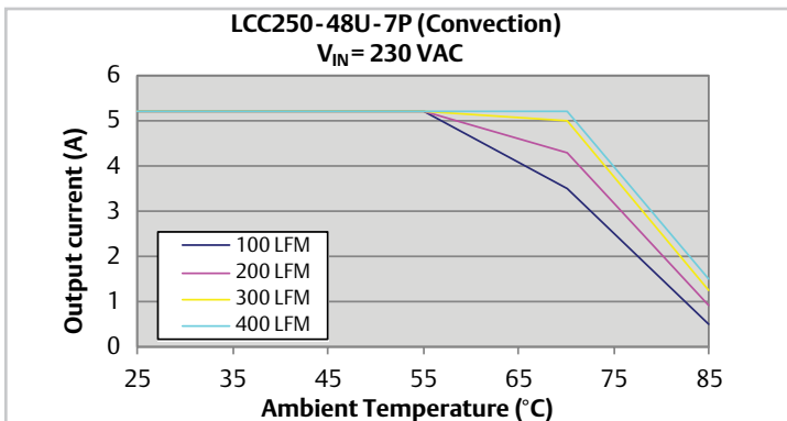
Fig 11. 48 V “7P” Suffix (Convection) Output Current Derating at 230 Vac
