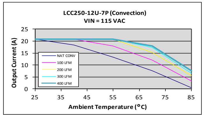
Fig 2. 12 V "7P" Suffix (Convection) Output Current Derating at 115 Vac
