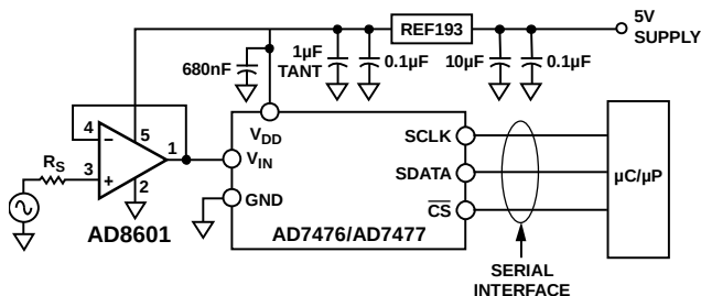
Figure 59. A Complete 3\text{ V} 12-Bit 1\text{ MHz} Analog-to-Digital Conversion System
