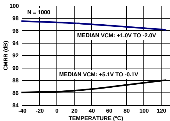
FIGURE 39. ISL28194 CMRR vs TEMPERATURE, V_{CM} = +1.0V \text{ TO } -2.0V, +5.1V \text{ TO } -0.1V
