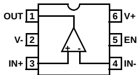
ISL28194, ISL28195 (6 LD 1.6X1.6X0.5 μTDFN) TOP VIEW
