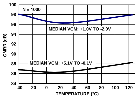
FIGURE 40. ISL28195 CMRR vs TEMPERATURE, V_{CM} = +1.0V \text{ TO } -2.0V, +5.1V \text{ TO } -0.1V
