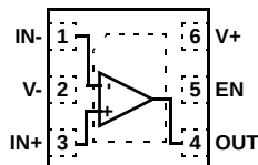
ISL28194, ISL28195 (6 LD 1.6X1.6X0.5 μTDFN) TOP VIEW
