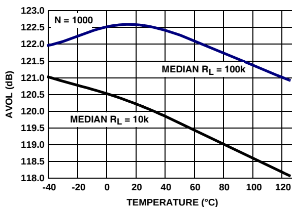
FIGURE 44. ISL28195 AVOL vs TEMPERATURE, V_+ = 5V
