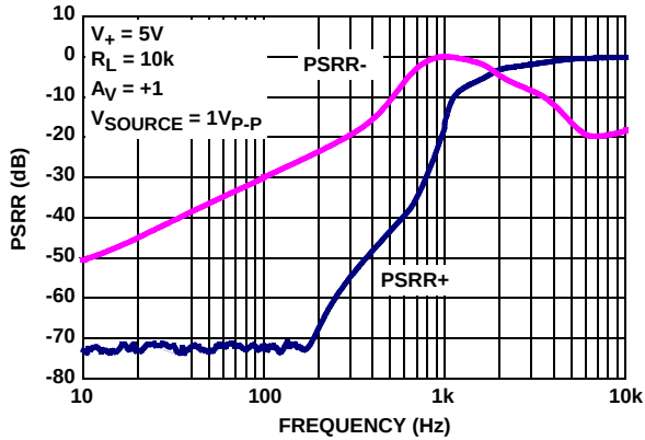
FIGURE 5. ISL28194 PSRR vs FREQUENCY
