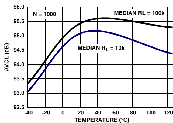
FIGURE 46. ISL28195 AVOL vs TEMPERATURE, V_+ = 1.8V
