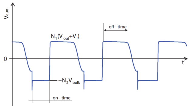
Figure 63. The signal obtained on the auxiliary winding swings negative during the on-time
