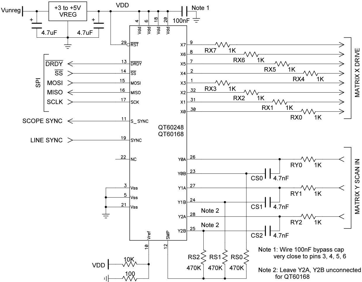
Figure 2.7 Wiring Diagram See Table 2.2 for further connection information.
