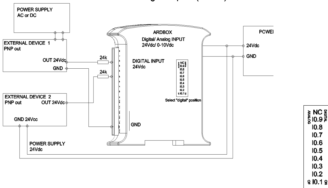
Switch configuration (Select digital position)
