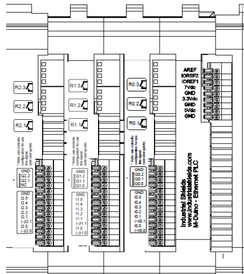
Input Pinout Output Pinout
