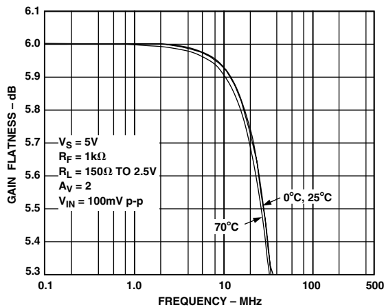
TPC 3. 0.1 dB Flatness vs. Frequency Over Temperature; V_S = 5V
