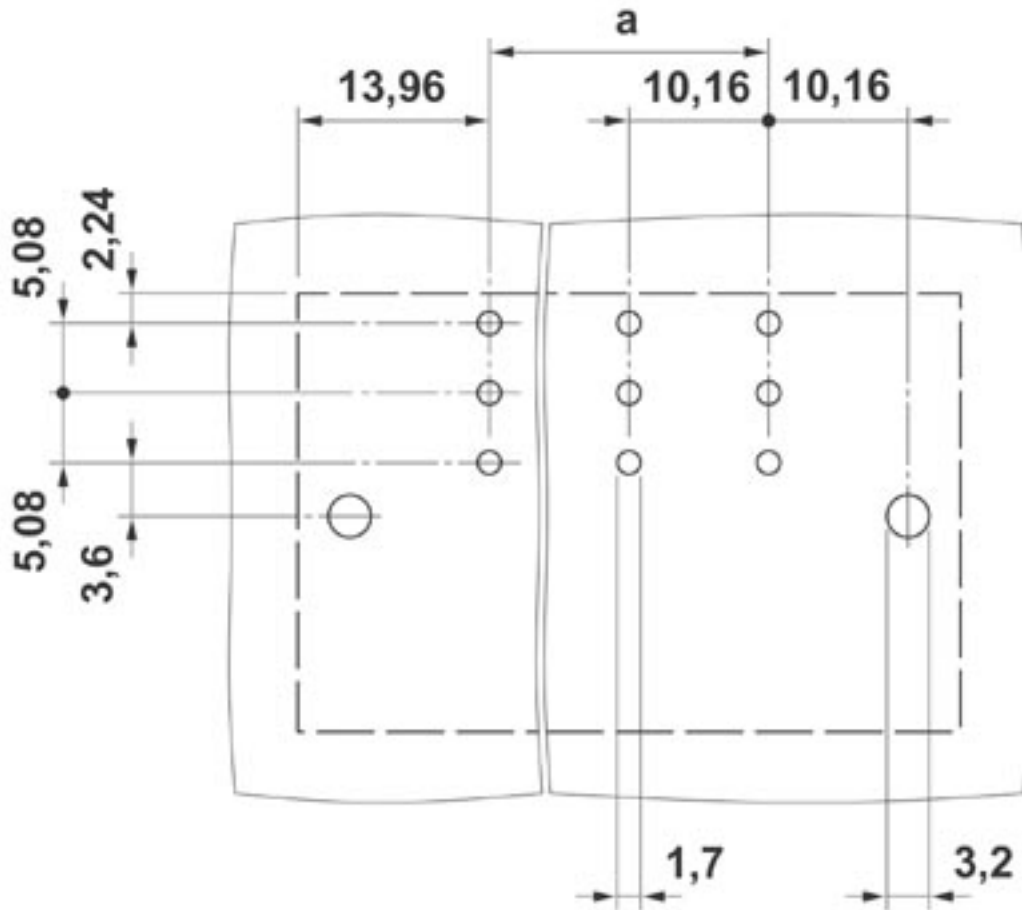
Drilling diagram
