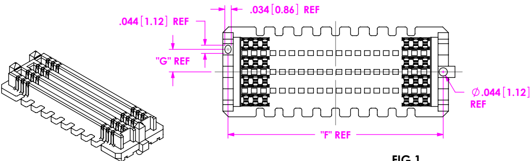
FIG 1 -08: 8 ROW (SEAM-30-02.0-XX-08-1-A-XX-K-TR SHOWN) (SOME CENTER FEATURES REMOVED FOR CLARITY)
