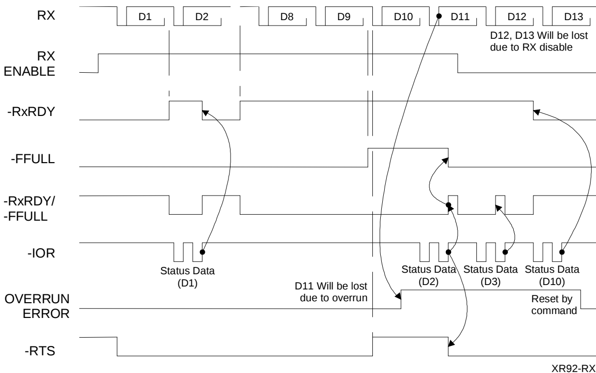
Figure 6: Receive Timing
