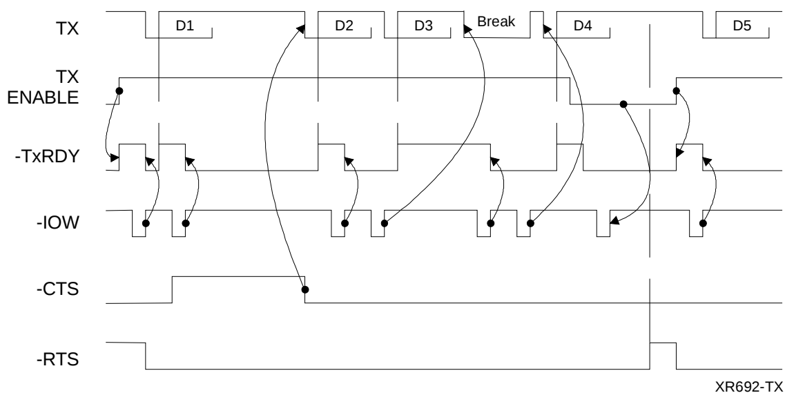
Figure 7: Transmit Timing
