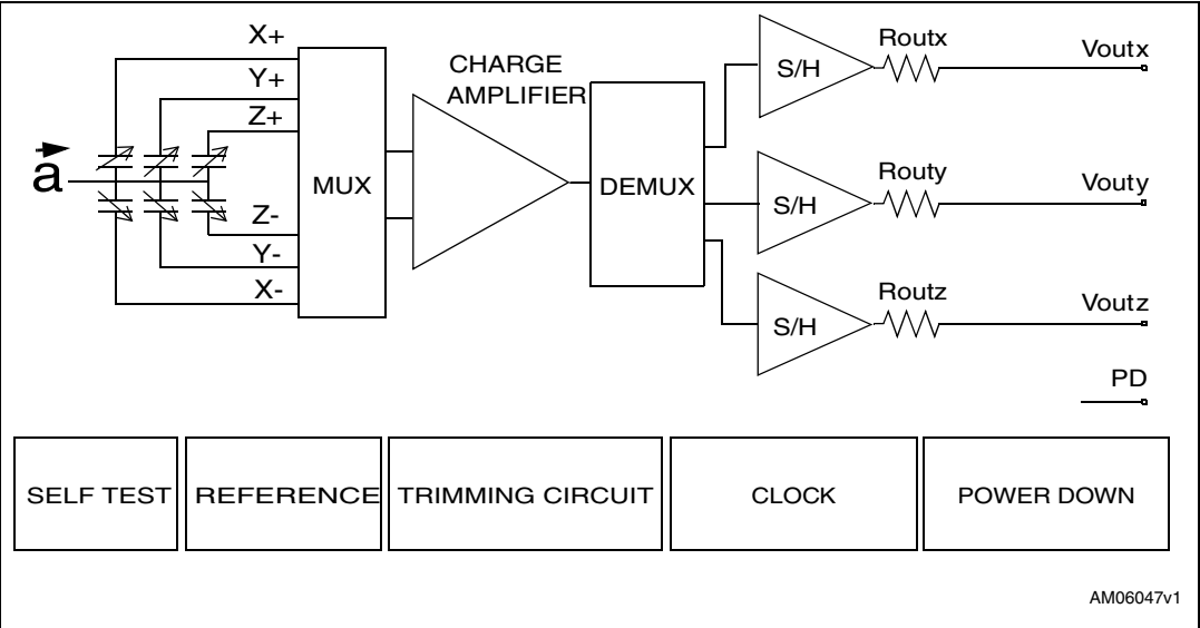
Figure 1. Block diagram
