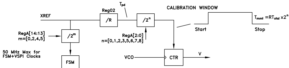
Figure 31. VCO Calibration
