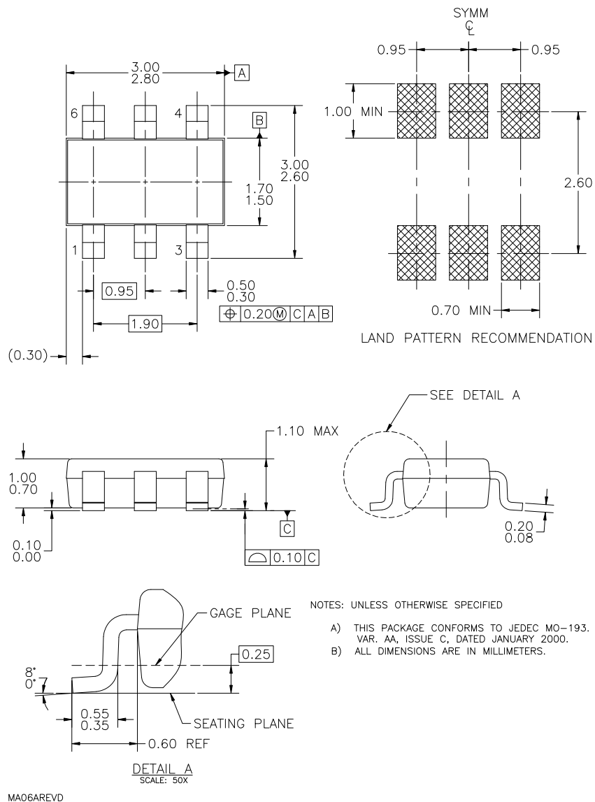
Figure 3. 6-LEAD, SUPERSOT6, JDEC MO-193, 1.6 MM WIDE (ACTIVE)
