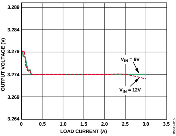
Figure 17. Load Regulation
