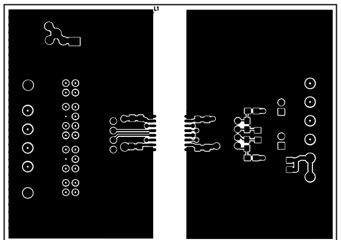
Figure 4. Top Layer
