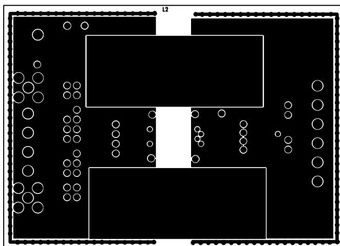
Figure 6. Internal Layer 2
