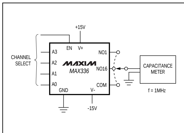
Figure 8. NO/COM Capacitance
