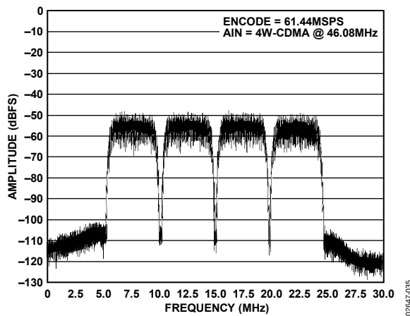
Figure 29. Four W-CDMA Carriers @ 46.08 MHz, Encode = 61.44 MSPS
