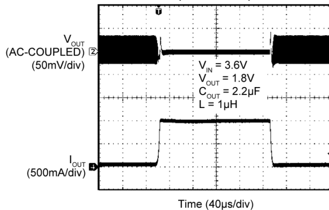
Load Transient (50mA to 1A)
