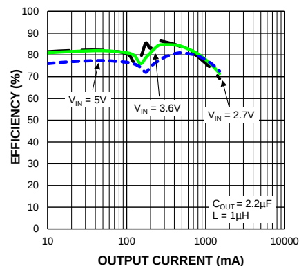
Efficiency ( V_{OUT} = 1.0V ) vs. Output Current
