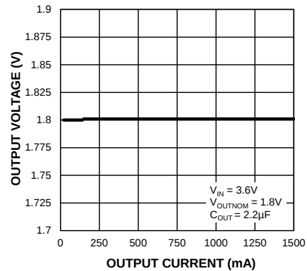
Load Regulation
