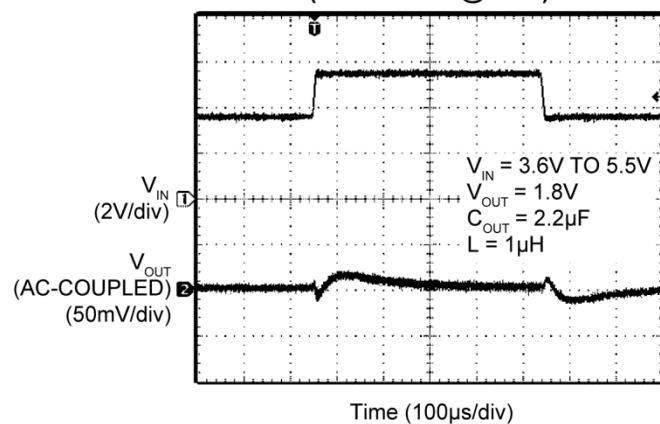
Line Transient (3.6V to 5.5V @ 1.5A)
