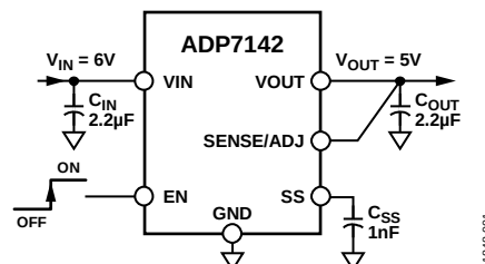
Figure 1. ADP7142 with Fixed Output Voltage, 5 V
