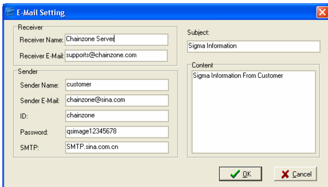
Fig. 5.14 E-Mail Setting
