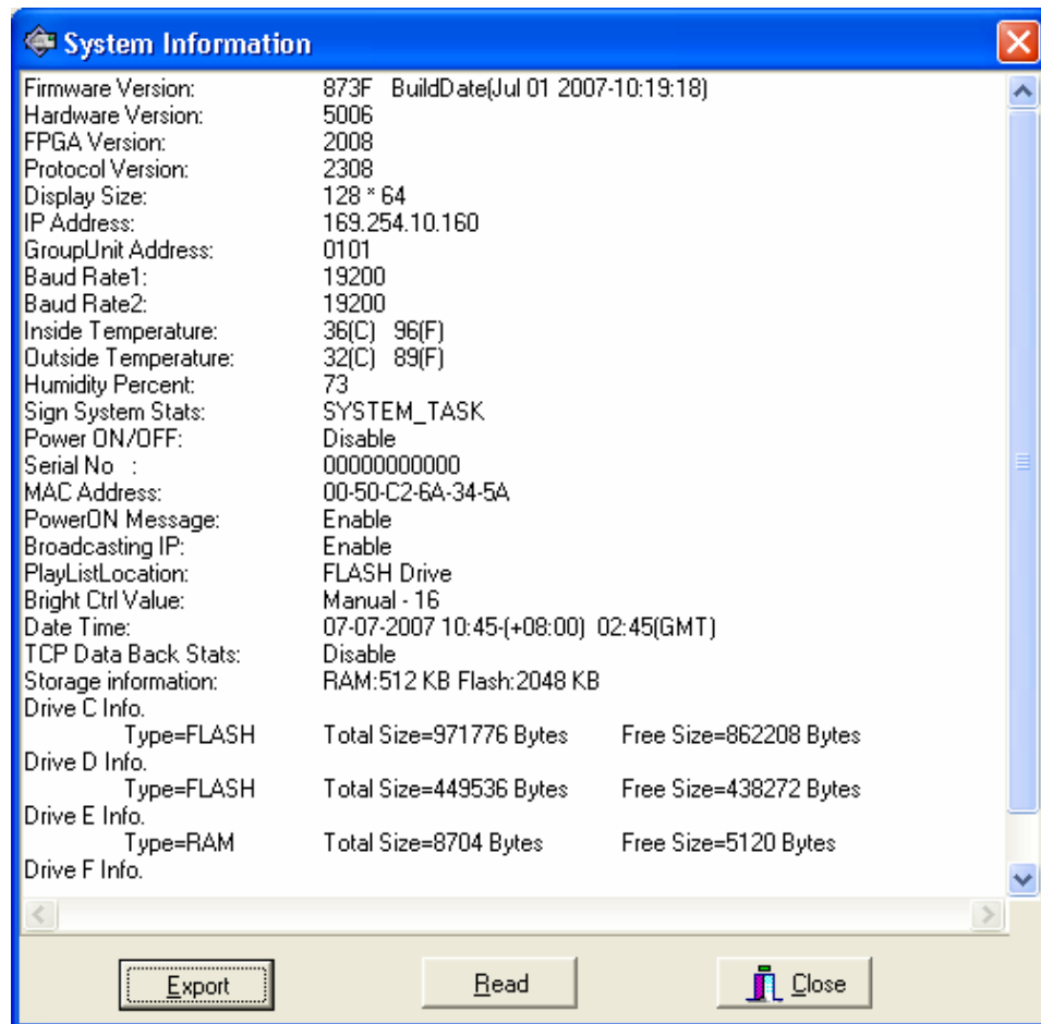
Fig. 5.25 System Information
