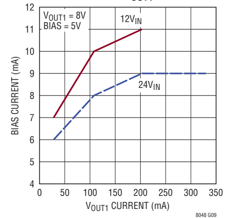
BIAS Current vs V_{OUT1} Load
