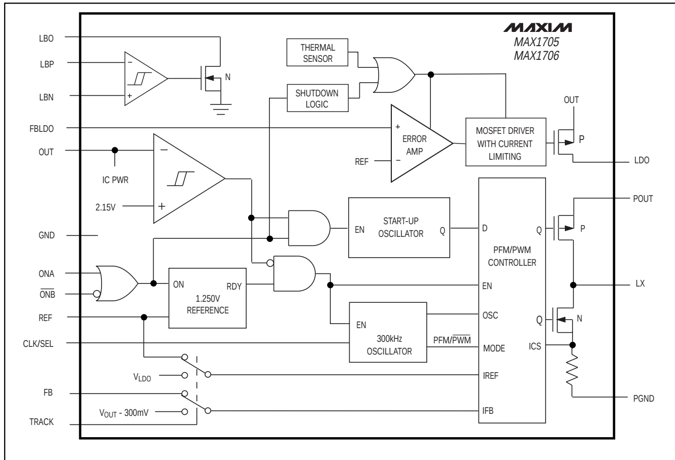
Figure 1. Functional Diagram
