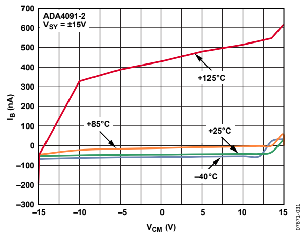
Figure 31. Input Bias Current vs. Common-Mode Voltage
