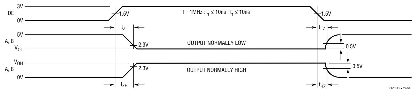
Figure 6. Driver Enable and Disable Times
