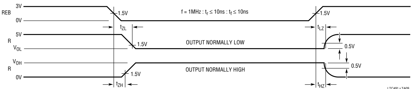
Figure 8. Receiver Enable and Disable Times
