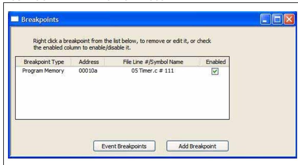
FIGURE 3-34: BREAKPOINTS DIALOGUE
