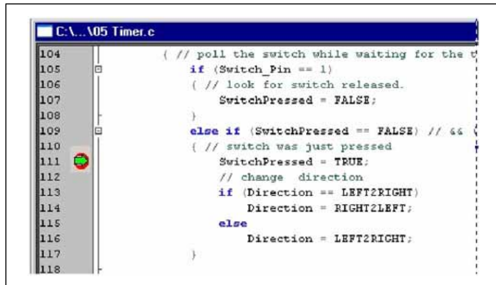
FIGURE 3-33: BREAKPOINT HALT
