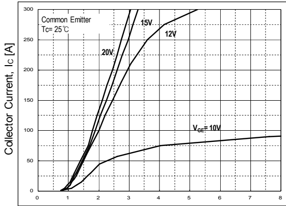
Collector - Emitter Voltage, V_{CE(sat)} [V] Fig 1. Typical Output characteristics
