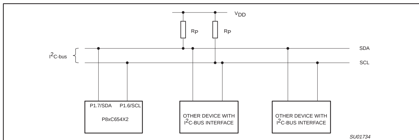
Figure 21. Typical I²C-bus configuration
