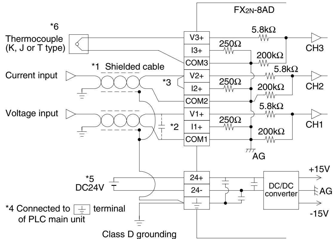
Figure 6.2: Wiring
