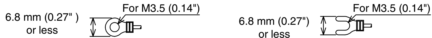
Figure 6.3: Crimp Terminals
