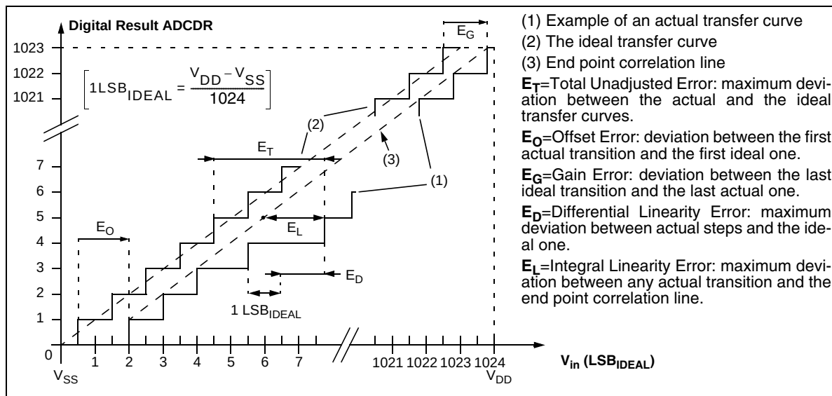
Figure 65. ADC Accuracy Characteristics
