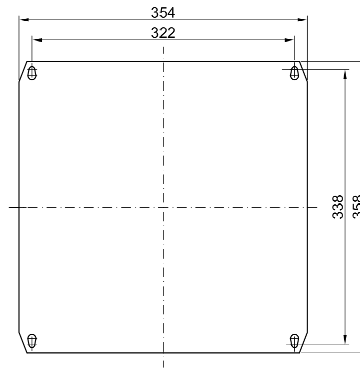
Base Plate
