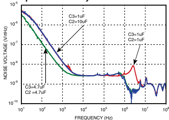
Figure 1. Vout=5V Output Noise Spectral Density [1]
