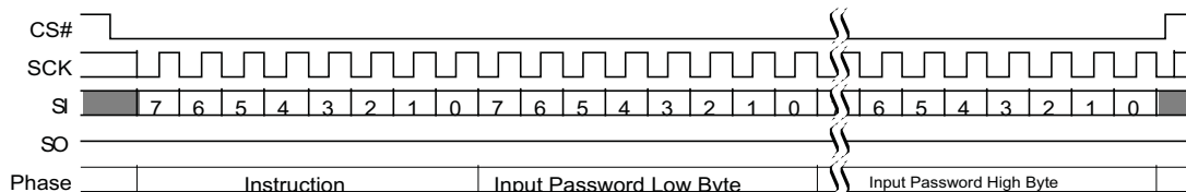
Figure 9.71 Password Program (PASSP E8h) Command Sequence
