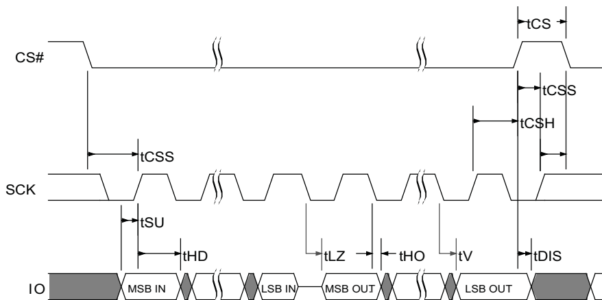
Figure 5.11 SPI SDR MIO Timing
