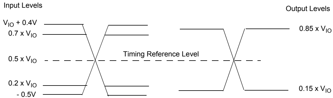
Figure 5.2 Input, Output, and Timing Reference Levels
