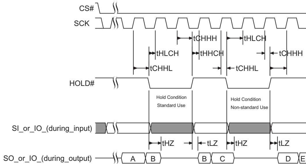
Figure 5.12 Hold Timing
