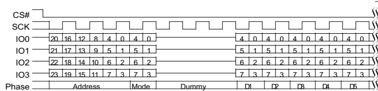
Figure 9.48 Continuous DDR Quad I/O Read Subsequent Access (3-Byte Address, HPLC=11b)
