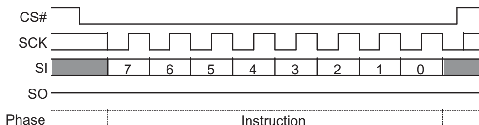
Figure 9.13 Write Enable (WREN 06h) Command Sequence
