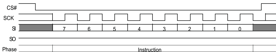
Figure 3.3 Stand Alone Instruction Command
