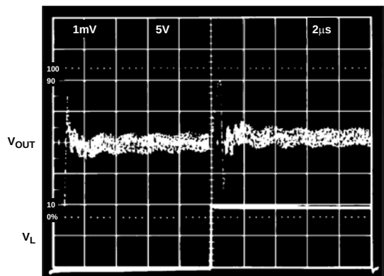
Figure 28. Load Crosstalk
