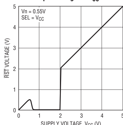
RST Output Voltage vs V_{CC}
