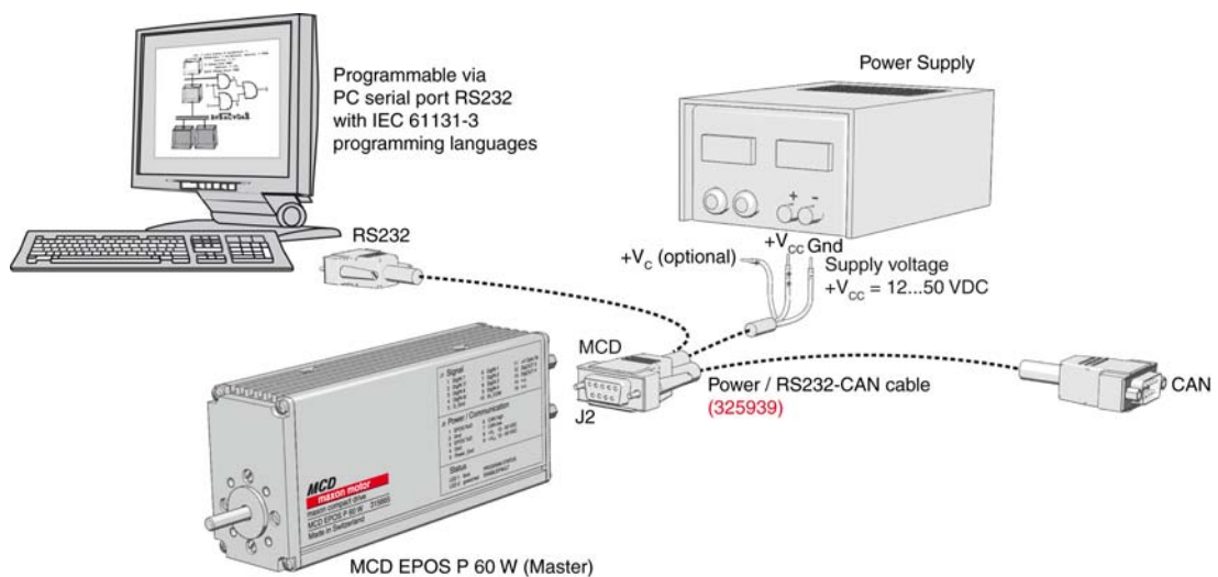
Figure 3-2 Minimum Wiring
