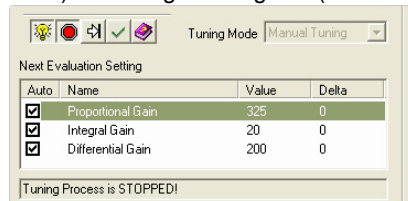
Figure 3-33 Next Evaluation Setting
