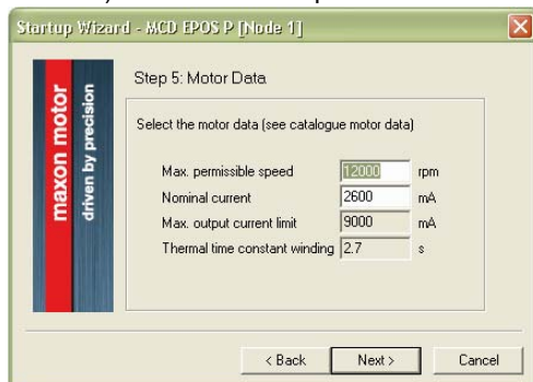
Figure 3-12 Startup Wizard Dialog: Motor Data
