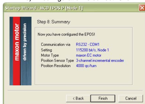
Figure 3-15 Startup Wizard Dialog: Configuration Summary
