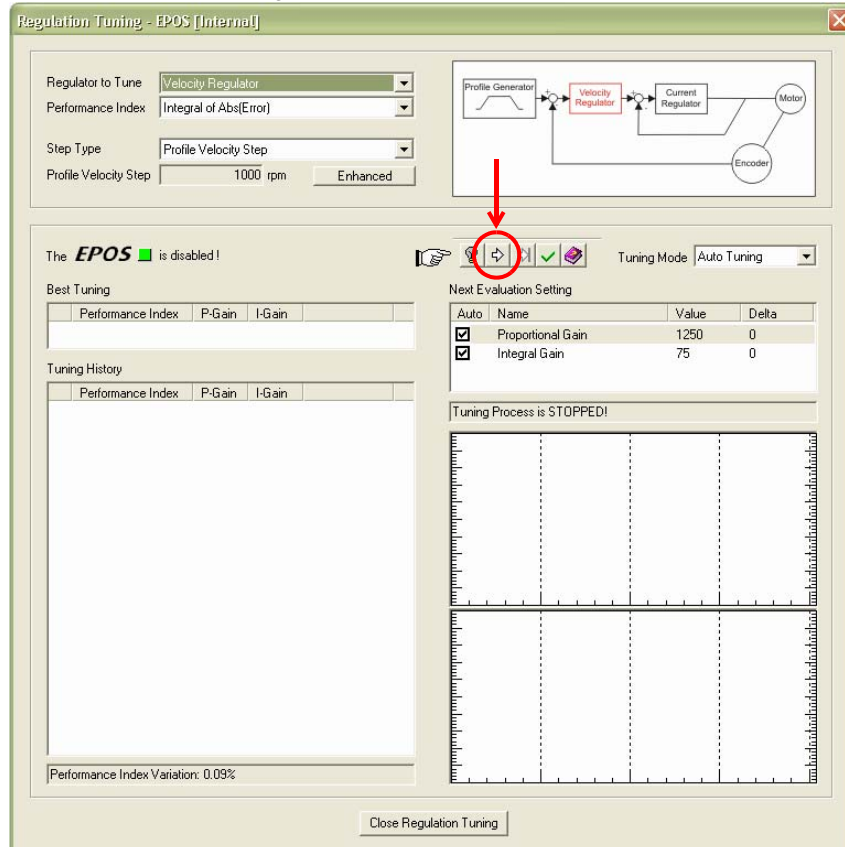
Figure 3-23 Auto Tuning of Velocity Regulator
