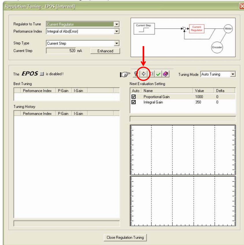
Figure 3-19 Auto Tuning of Current Regulator
