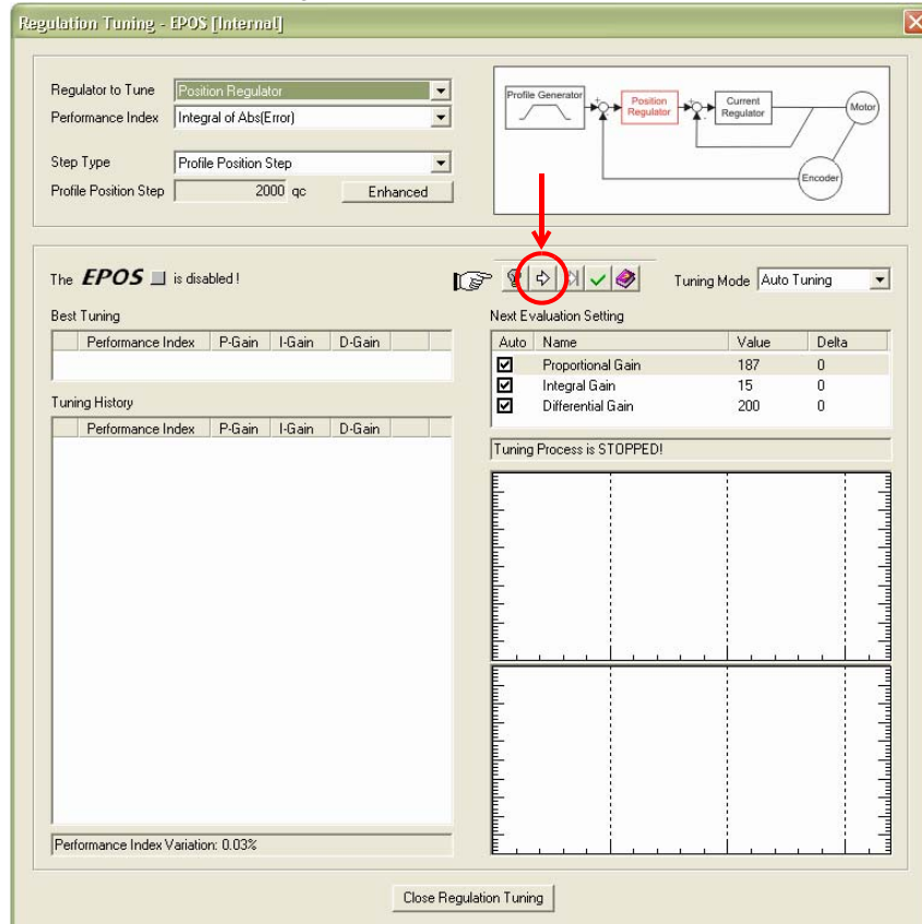
Figure 3-28 Auto Tuning of Position Regulator
