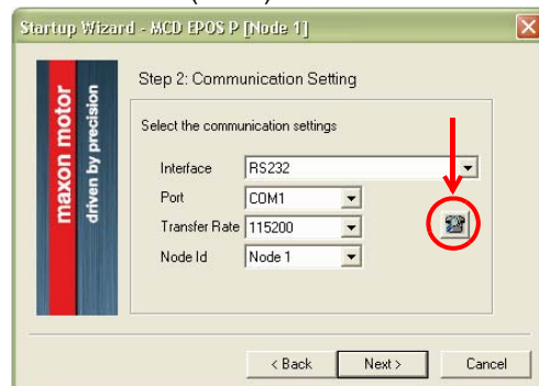
Figure 3-8 Startup Wizard Dialog: Communication Setting
