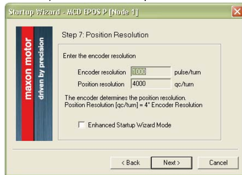
Figure 3-14 Startup Wizard Dialog: Position Resolution
